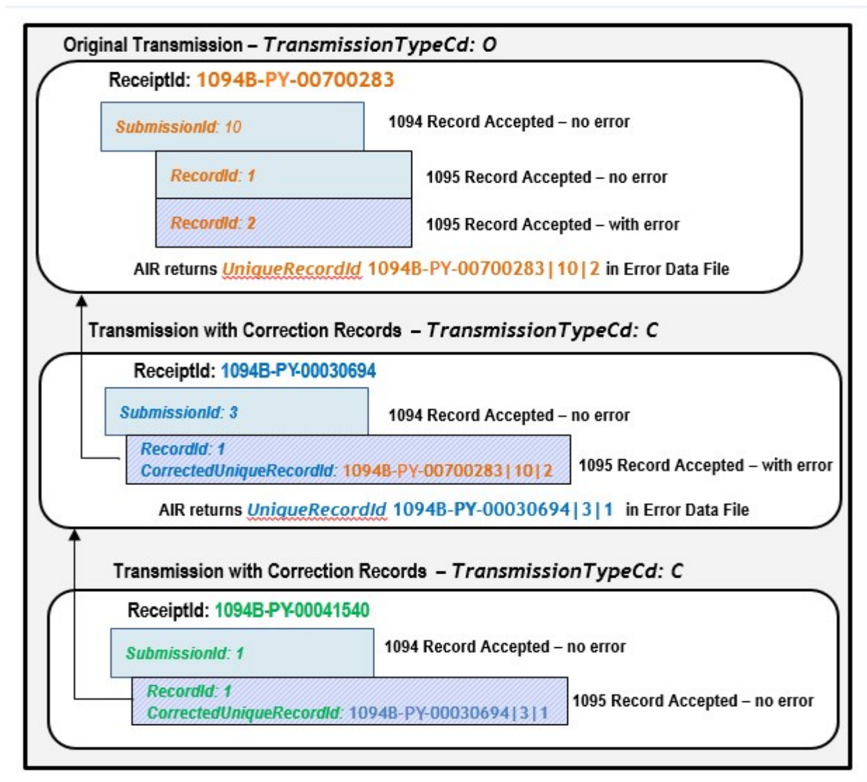
Figure 7-1: Reference Records to be Corrected
