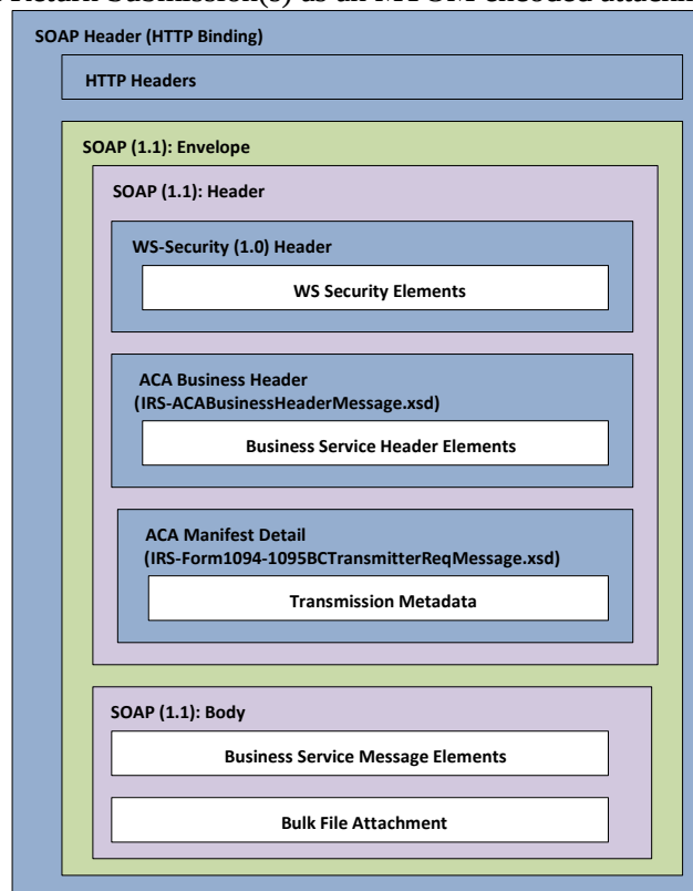
Figure 4-3: SOAP Message Structure
